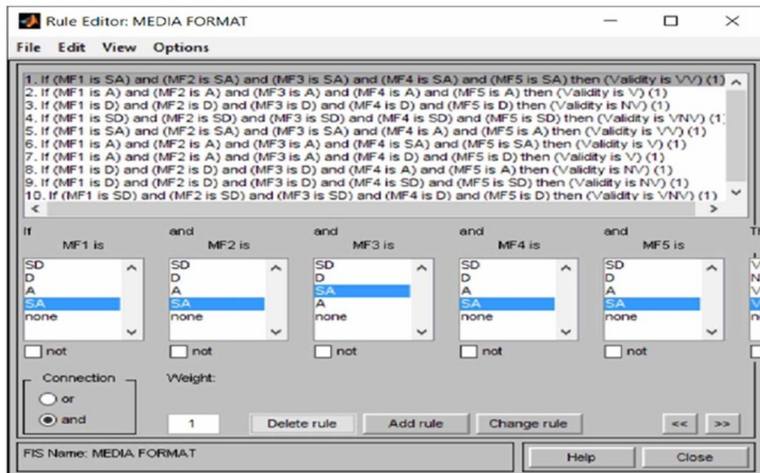
Figure 8. Fuzzy inference rule for media format
